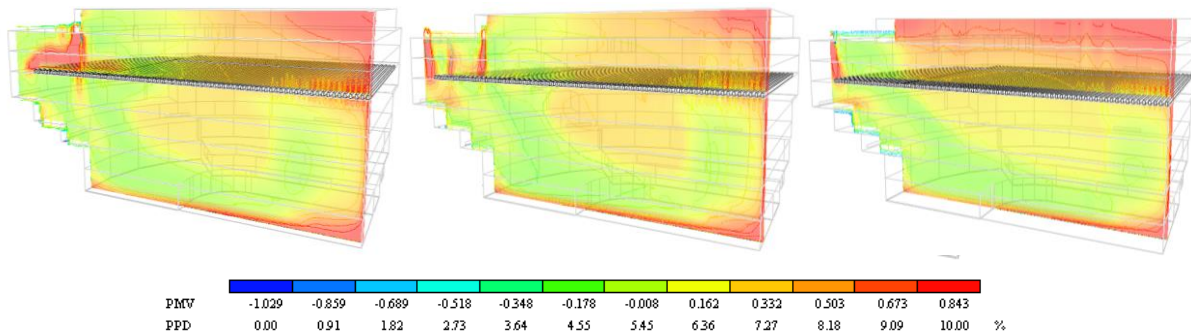
(a) (b) (c) Figure 9 (a) Option 1 (b) Option 4 (c) Option 5 PPD profile
