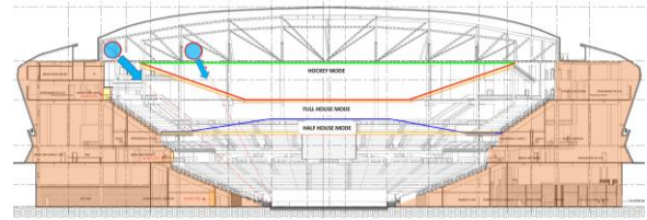
Figure 5 Option 4-Combination of OHAD from upper ring duct and outboard upper ring duct directed at one angle
