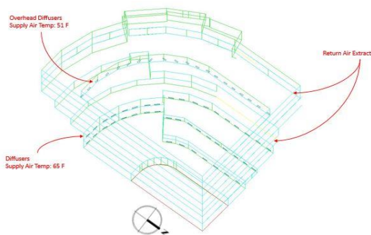
Figure 3 Supply diffusers and return air extracts
