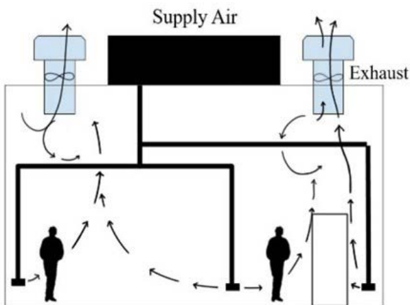
FIGURE 2. DISPLACEMENT VENTILATION
