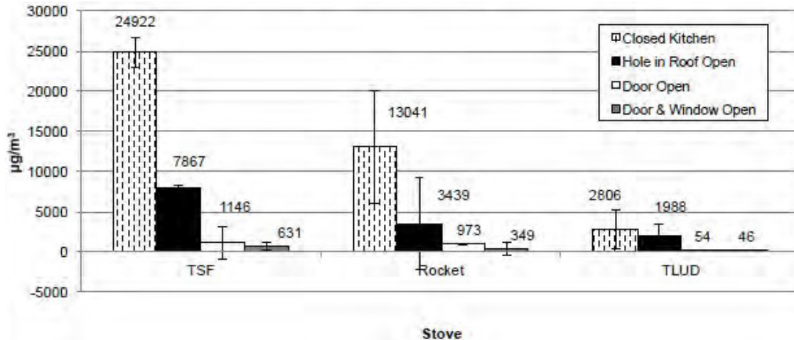
Figure D1 Mean PM 2.5 Concentrations by Stove in Test Kitchen.
