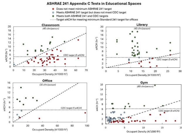
Figure 4 Equivalent air changes per hour from 241 Appendix C tests versus occupant density for various school spaces.
